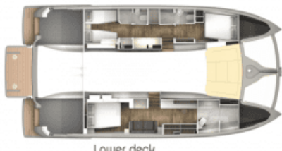
Lower deck
